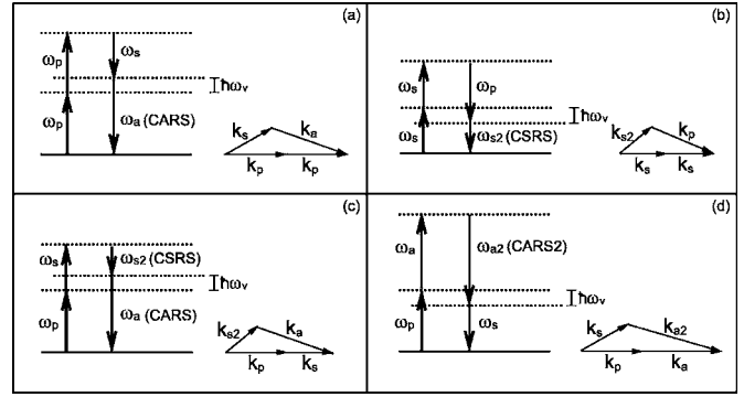
Fig. 2. Energy level diagrams for various four-wave mixing processes with virtual levels. Cases (a) and (b) represent typical coherent anti-Stokes (CARS) and Stokes (CSRS) Raman scattering processes, respectively. Cases (c) and (d) can exist for collinear pump and Raman-detuned beams. Both geometries are capable of producing CARS/CSRS spectra. The subscripts p , s , and a denote pump, Stokes, and anti-Stokes light, respectively, with numbers indicating the order of the Raman-shifted component with respect to \omega_p . The molecular vibrational frequency is denoted as \omega_v .
