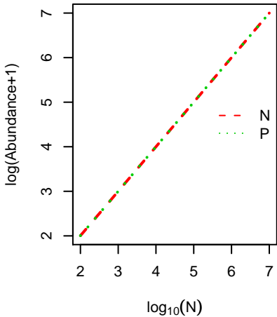
Initial Abundances (t=1)
