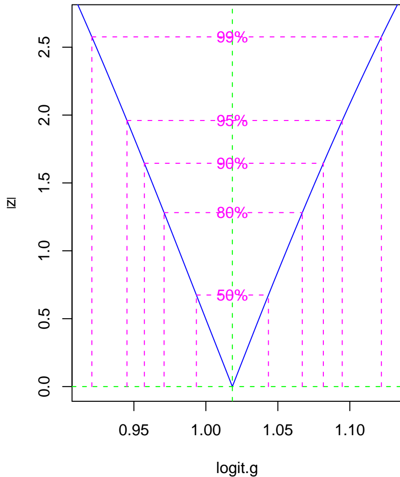
Likelihood profile: logit.g
