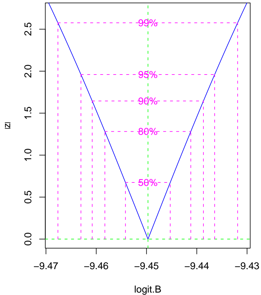
Likelihood profile: logit.B
