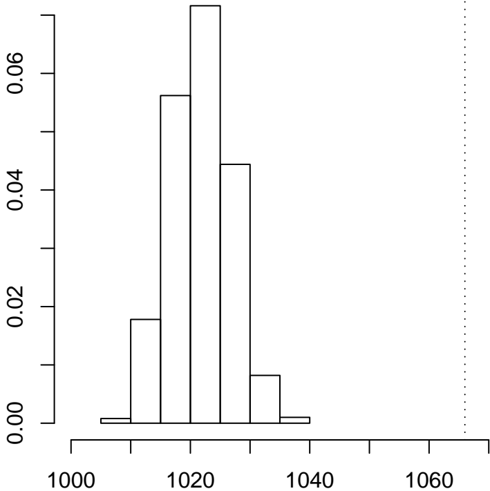
Histogram of unatt.sim
