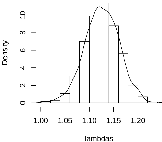
Histogram of lambdas
