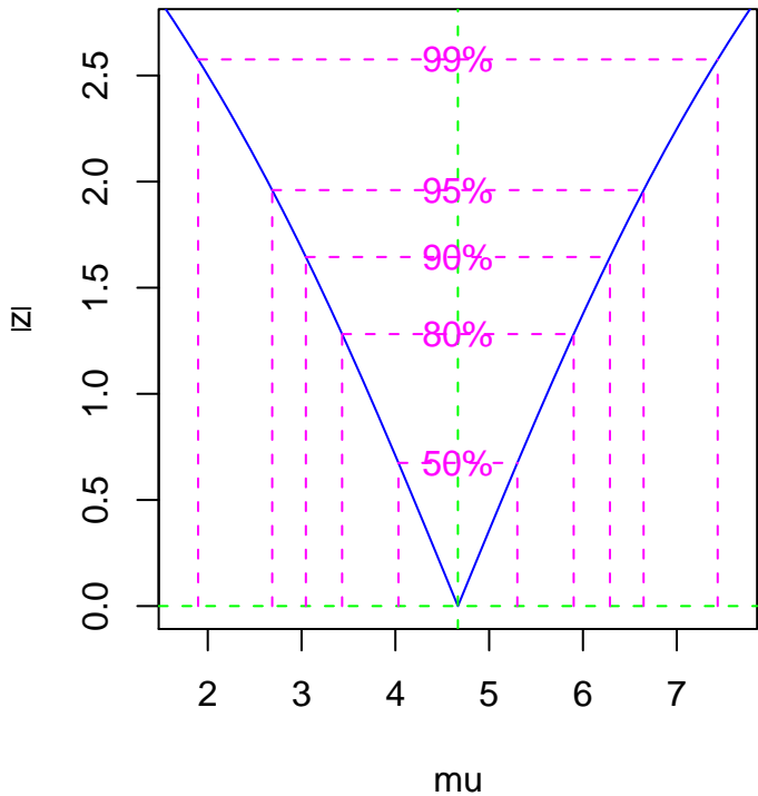
Likelihood profile: mu
