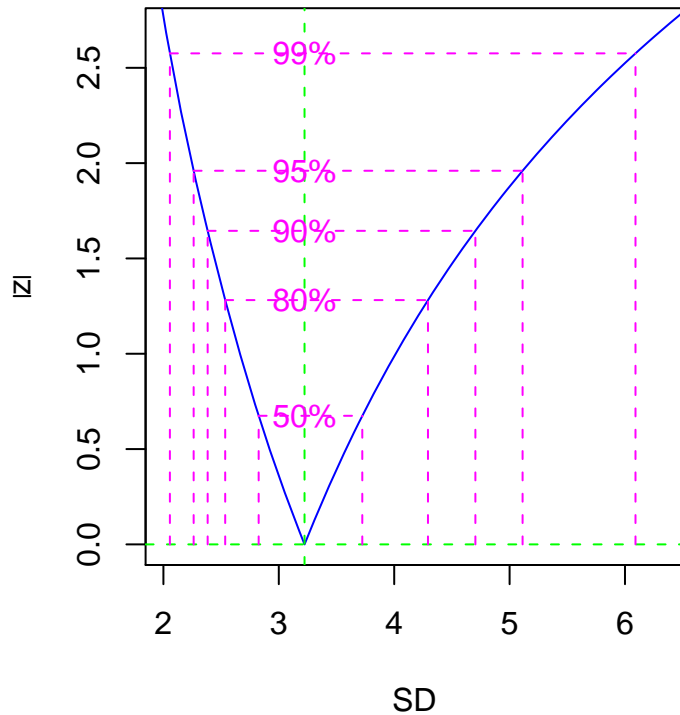
Likelihood profile: SD
